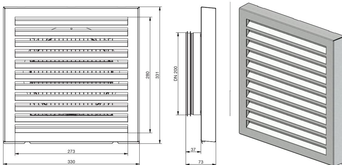
DN 200
